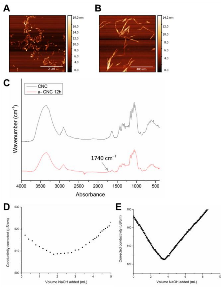
Supplementary Figure III-1 Morphological and chemical characterization of CNC and modified CNC. AFM images of modified CNC at 5x5 μm (A) and 0.5x0.5 μm (B). FTIR analysis of CNC and modified CNC (C). Conductometric titration curve of modified CNC to calculate the oxidation (D) and sulfation degree (E).
